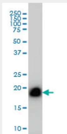
RHOA monoclonal antibody (M06), clone 1C10 Western Blot analysis of RHOA expression in A-431
